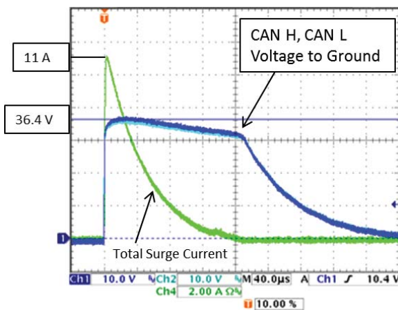
Figure 1 - CDSOT23-T24CAN Clamp Voltages for a +500 V Surge
